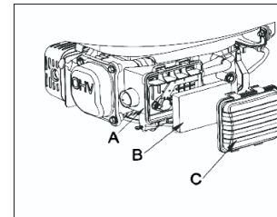
Fig. 10 A: Air cleaner case B: Foam element C: Air cleaner cover
